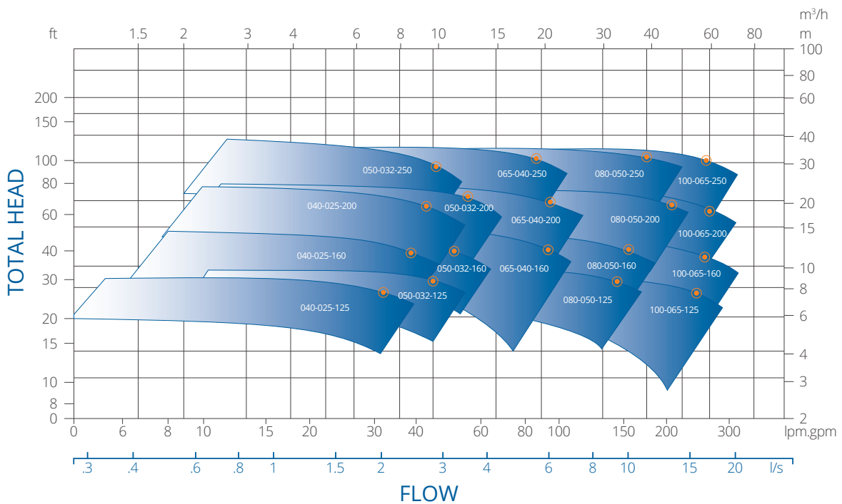
Selection Chart CRP-M CC
